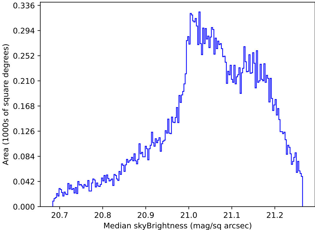
too_elab_r128_d3_ugrizy_v3.4_10yrs All sky r band: Median skyBrightness
