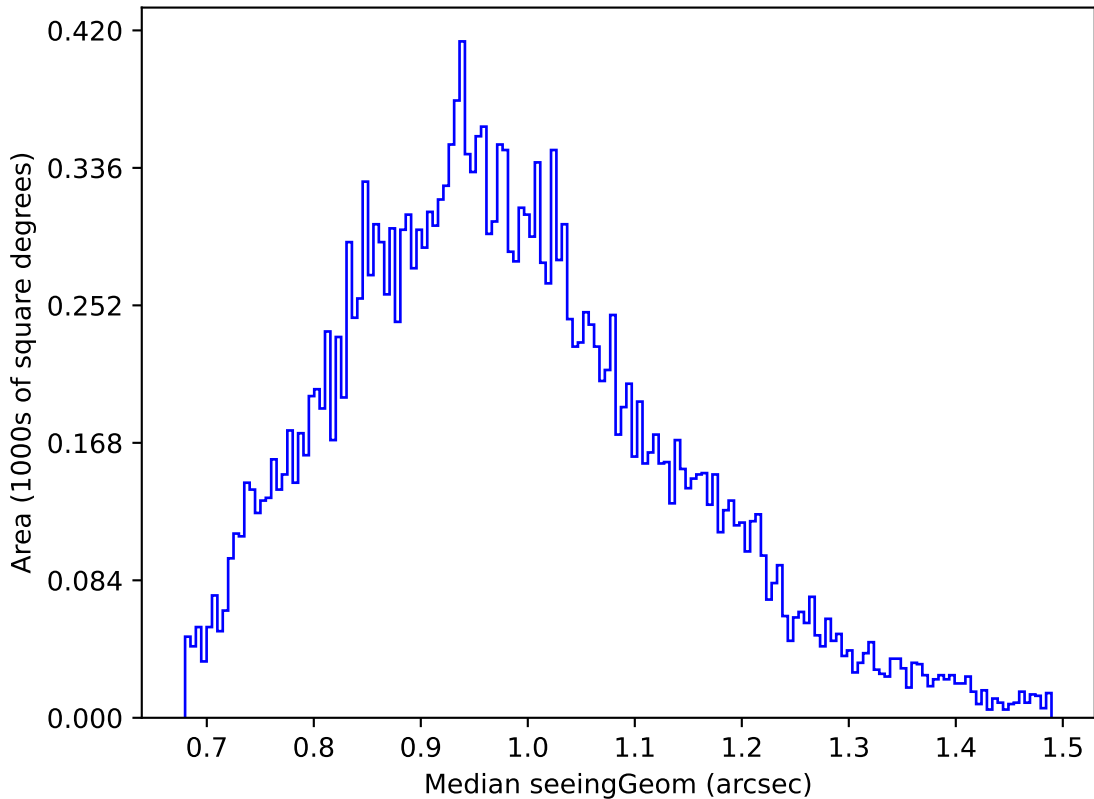
too_elab_r128_d3_ugrizy_v3.4_10yrs Yr 1 u band: Median seeingGeom
