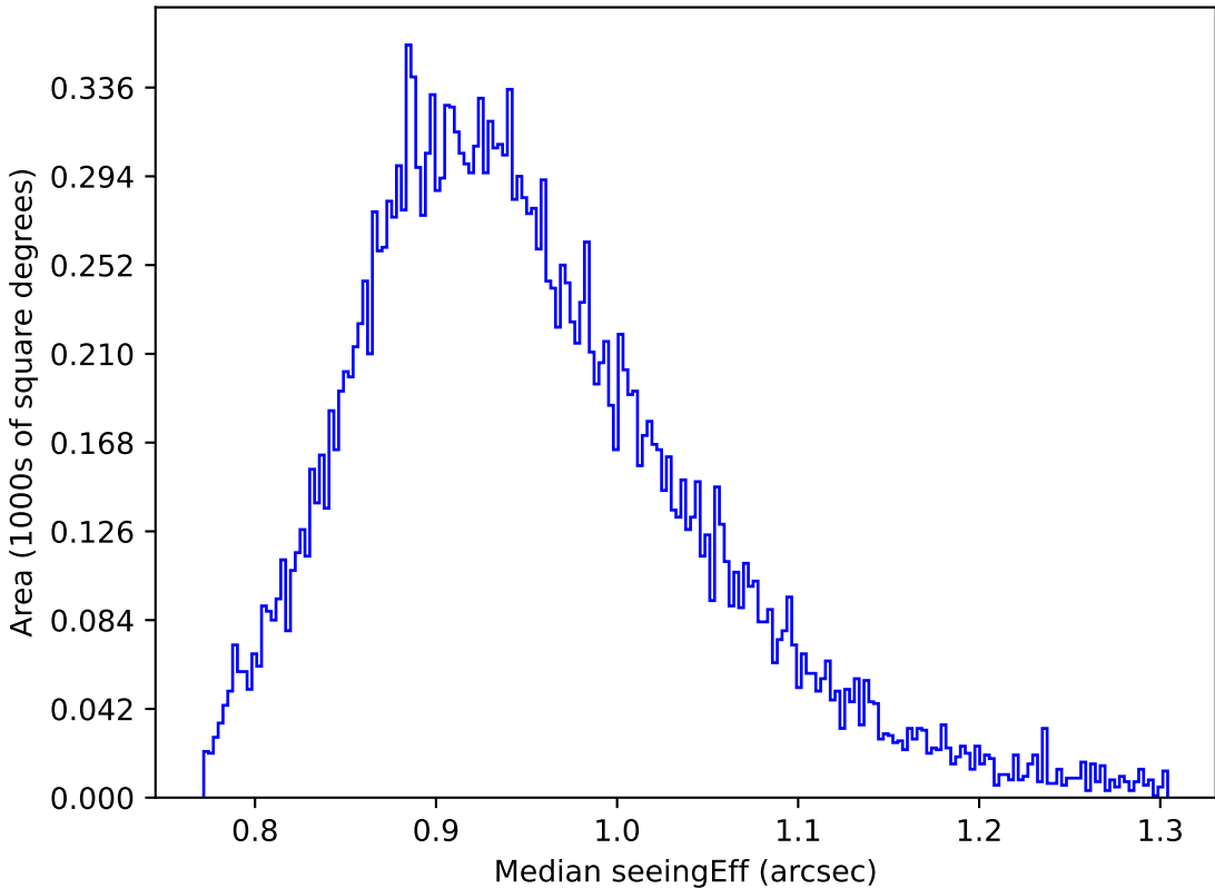
too_elab_r128_d3_ugrizy_v3.4_10yrs Yr 1 y band: Median seeingEff
