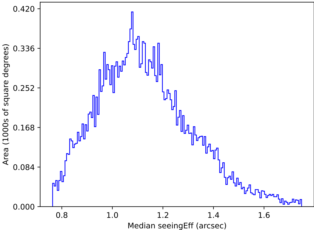
too_elab_r128_d3_ugrizy_v3.4_10yrs Yr 1 u band: Median seeingEff
