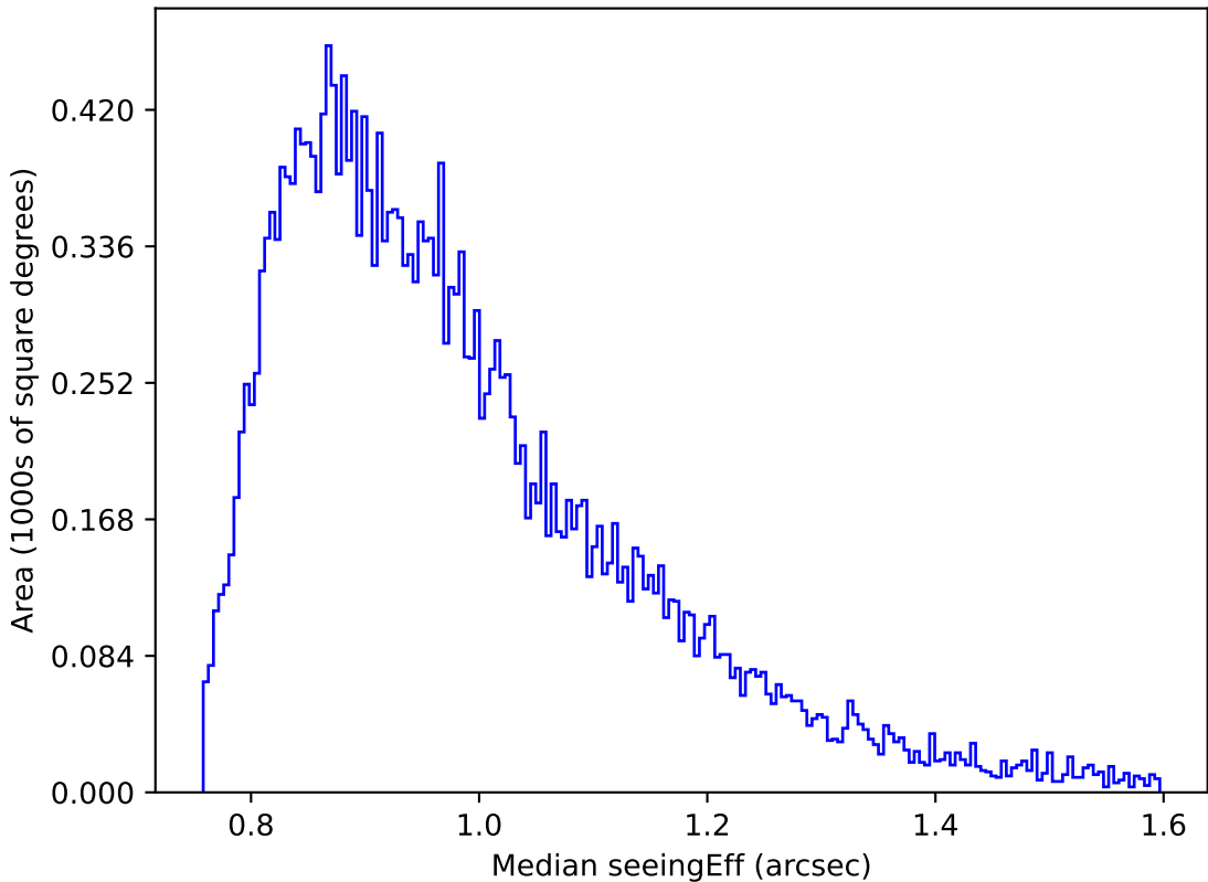
too_elab_r128_d3_ugrizy_v3.4_10yrs Yr 1 r band: Median seeingEff
