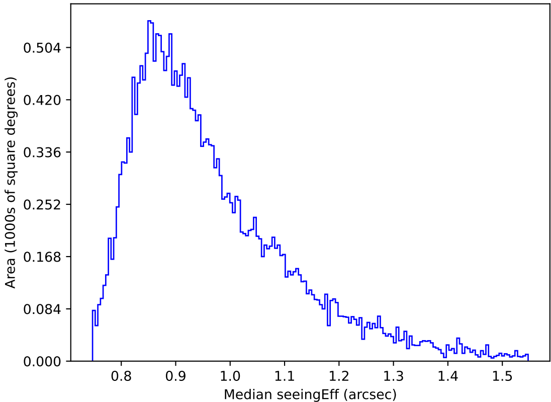
too_elab_r128_d3_ugrizy_v3.4_10yrs Yr 1 i band: Median seeingEff
