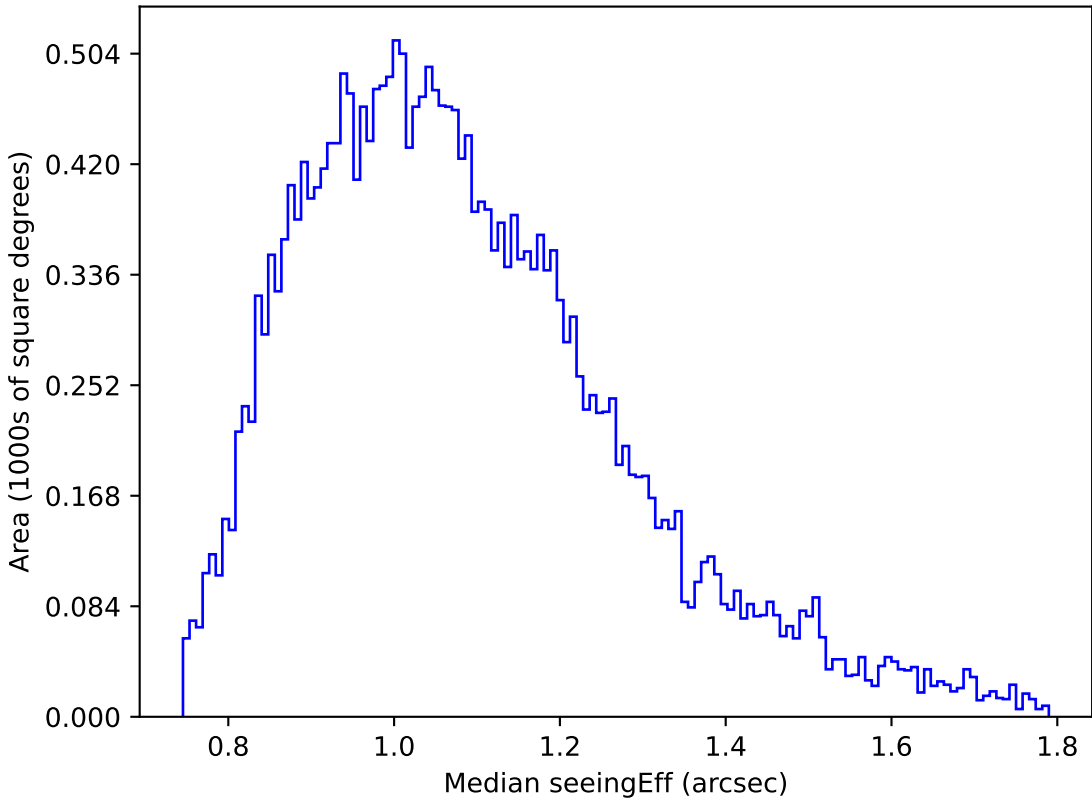
too_elab_r128_d3_ugrizy_v3.4_10yrs Yr 1 g band: Median seeingEff
