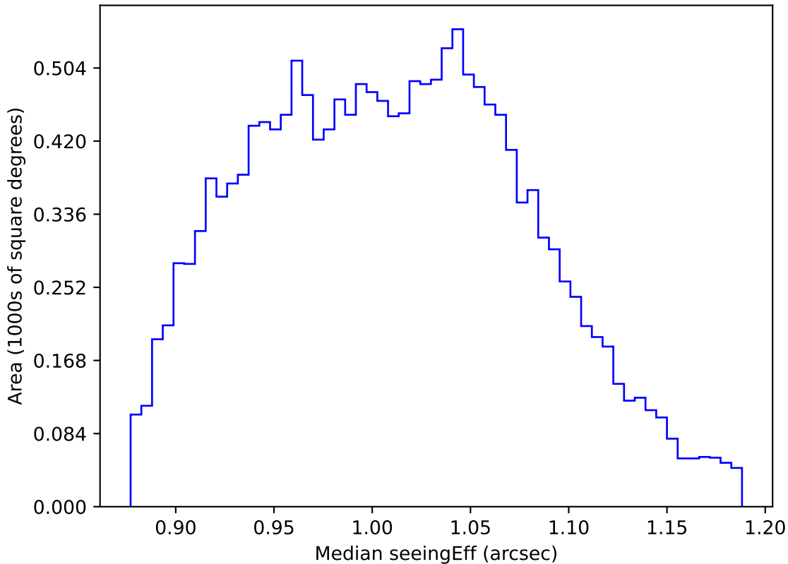
too_elab_r128_d3_ugrizy_v3.4_10yrs WFD z band: Median seeingEff
