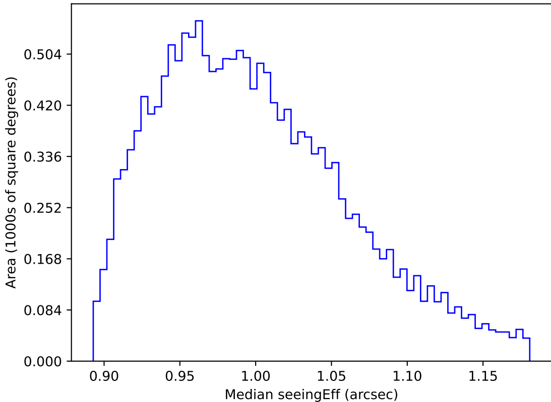
too_elab_r128_d3_ugrizy_v3.4_10yrs WFD y band: Median seeingEff
