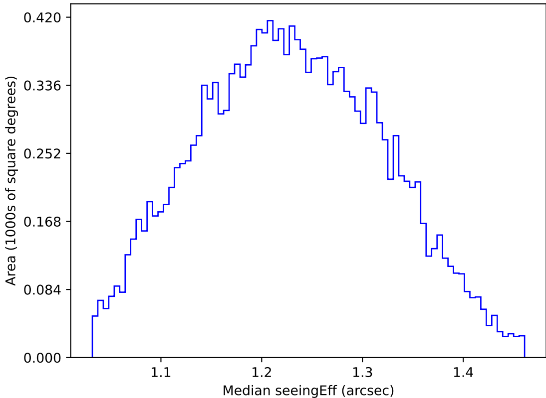
too_elab_r128_d3_ugrizy_v3.4_10yrs WFD u band: Median seeingEff
