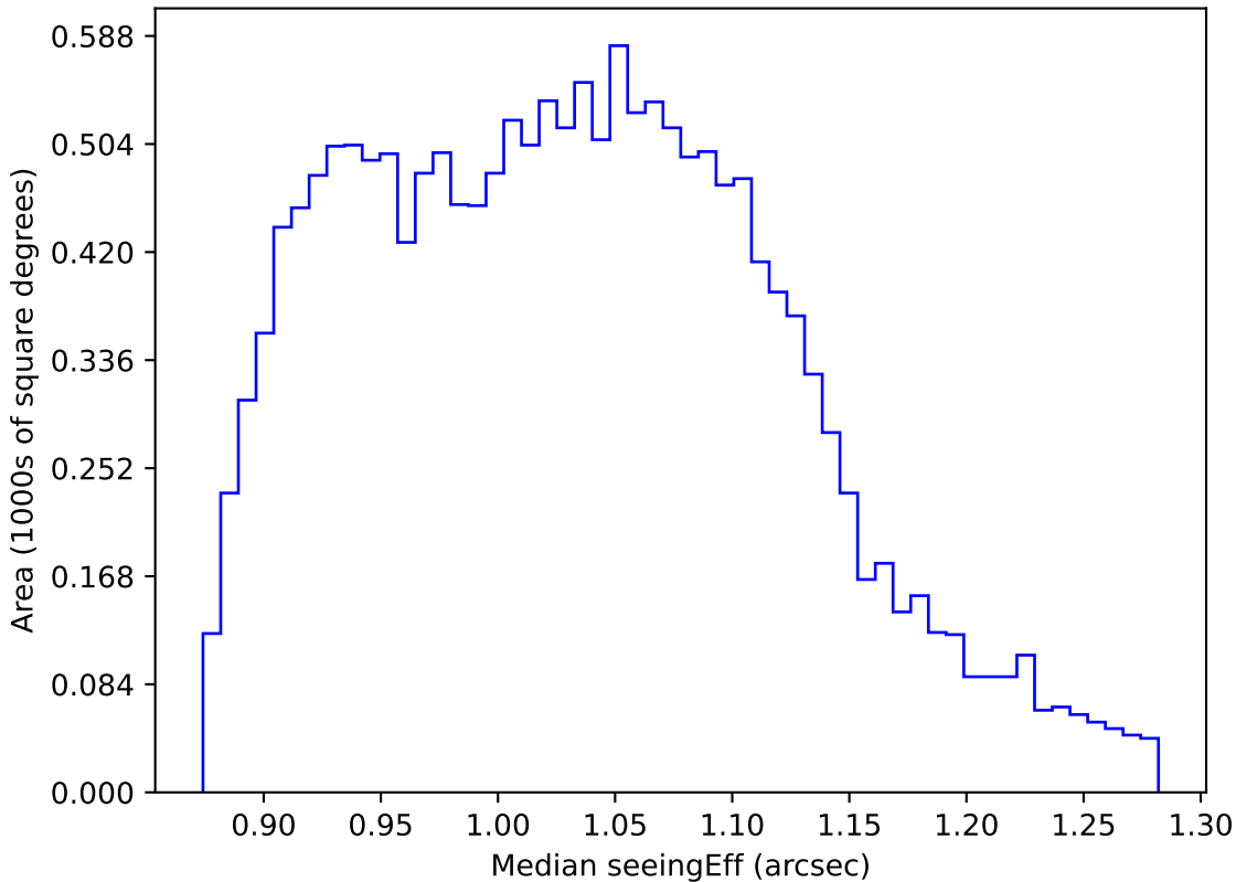
too_elab_r128_d3_ugrizy_v3.4_10yrs WFD r band: Median seeingEff
