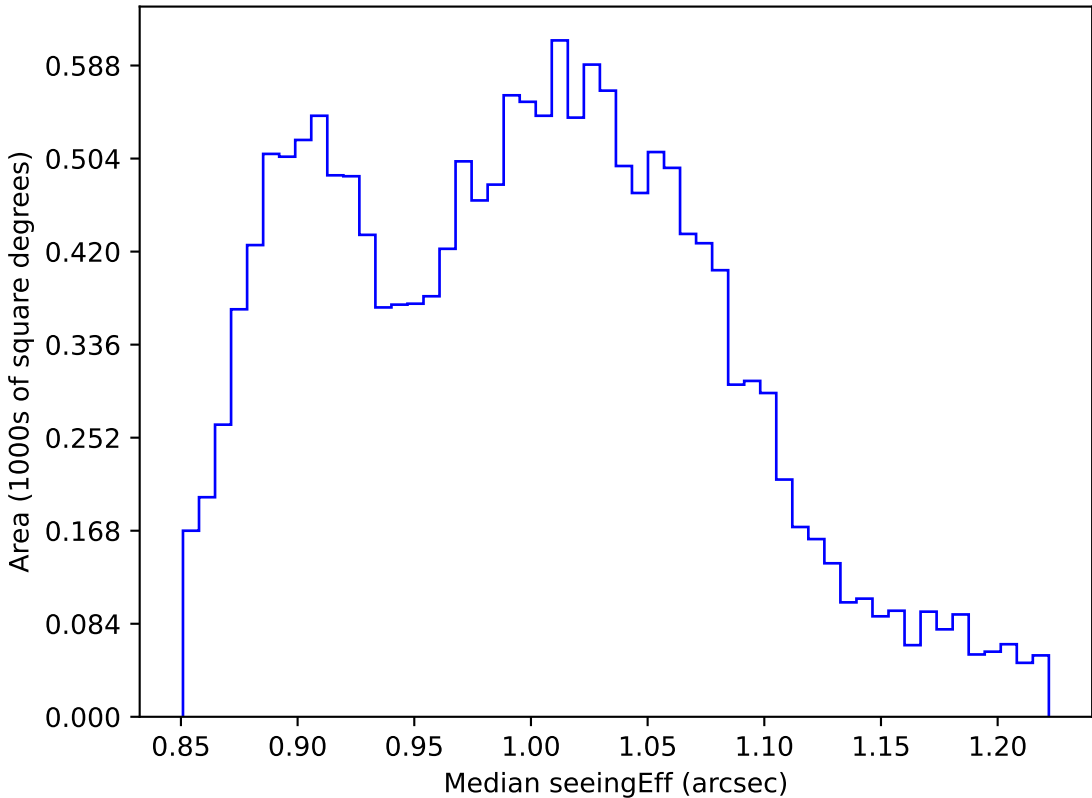
too_elab_r128_d3_ugrizy_v3.4_10yrs WFD i band: Median seeingEff
