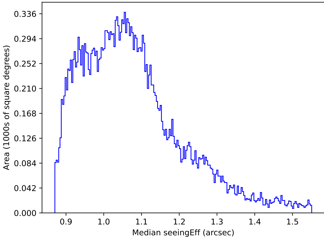
too_elab_r128_d3_ugrizy_v3.4_10yrs All sky r band: Median seeingEff
