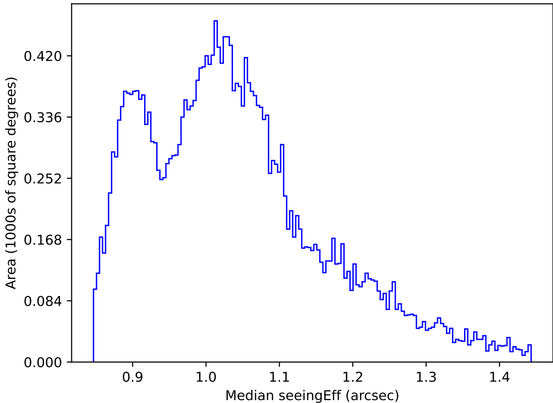
too_elab_r128_d3_ugrizy_v3.4_10yrs All sky i band: Median seeingEff
