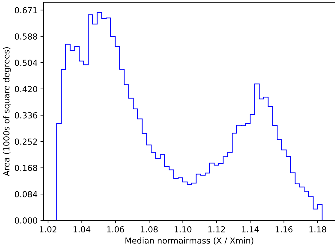
too_elab_r128_d3_ugrizy_v3.4_10yrs WFD all bands: Median normairmass
