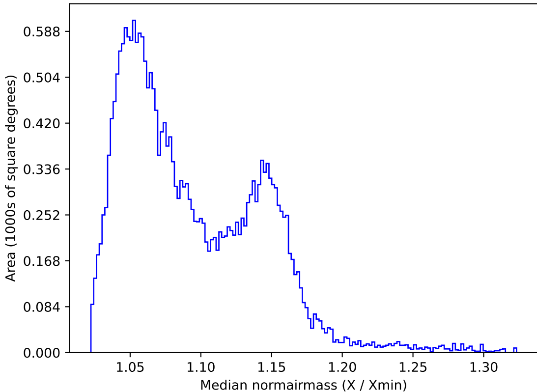
too_elab_r128_d3_ugrizy_v3.4_10yrs All sky y band: Median normairmass
