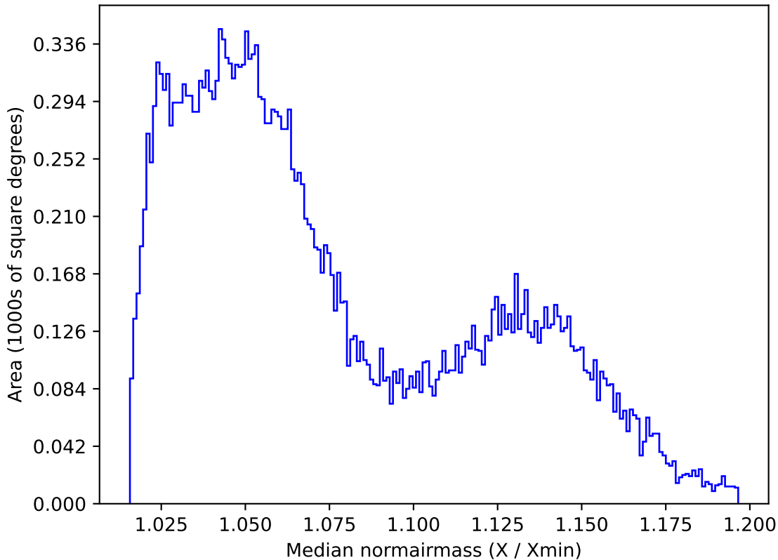
too_elab_r128_d3_ugrizy_v3.4_10yrs All sky r band: Median normairmass
