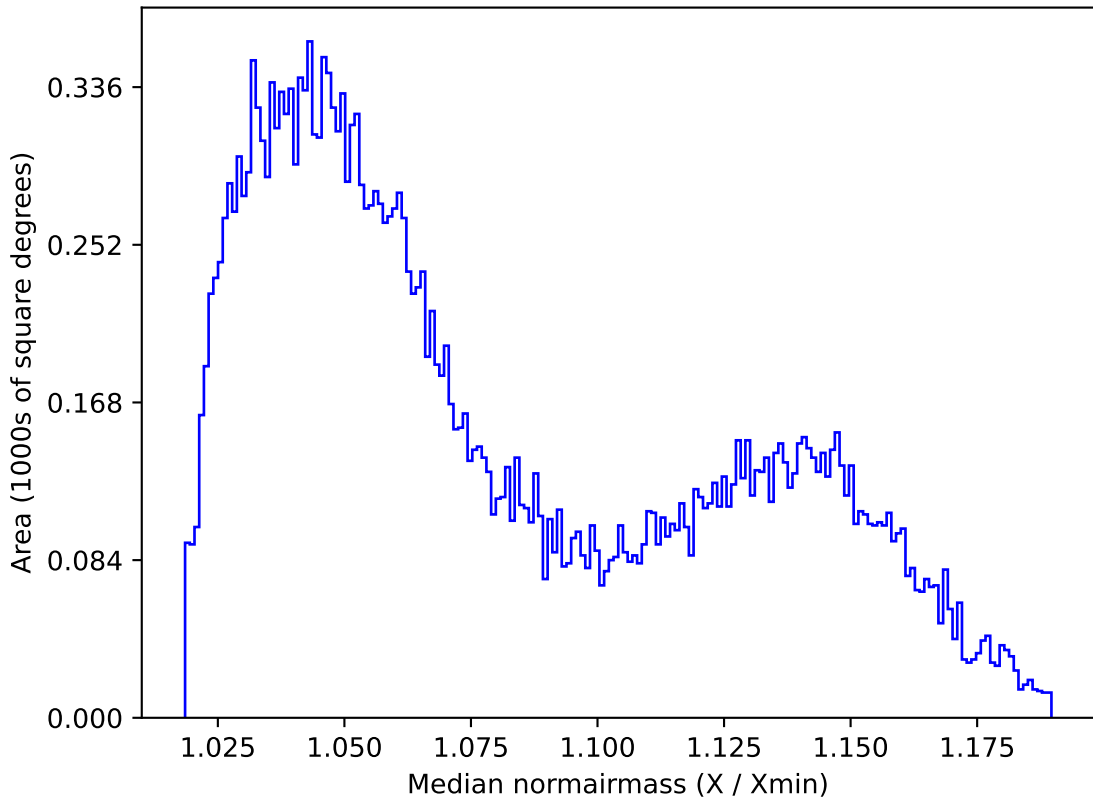
too_elab_r128_d3_ugrizy_v3.4_10yrs All sky i band: Median normairmass
