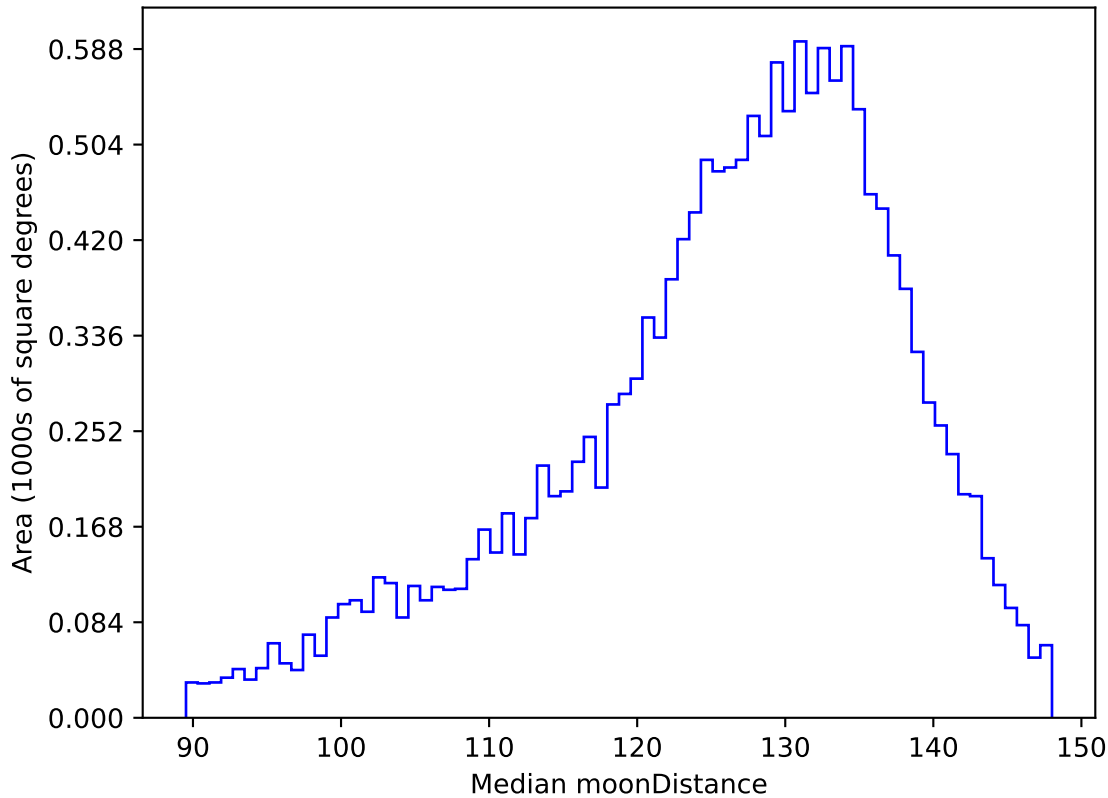
too_elab_r128_d3_ugrizy_v3.4_10yrs WFD u band: Median moonDistance
