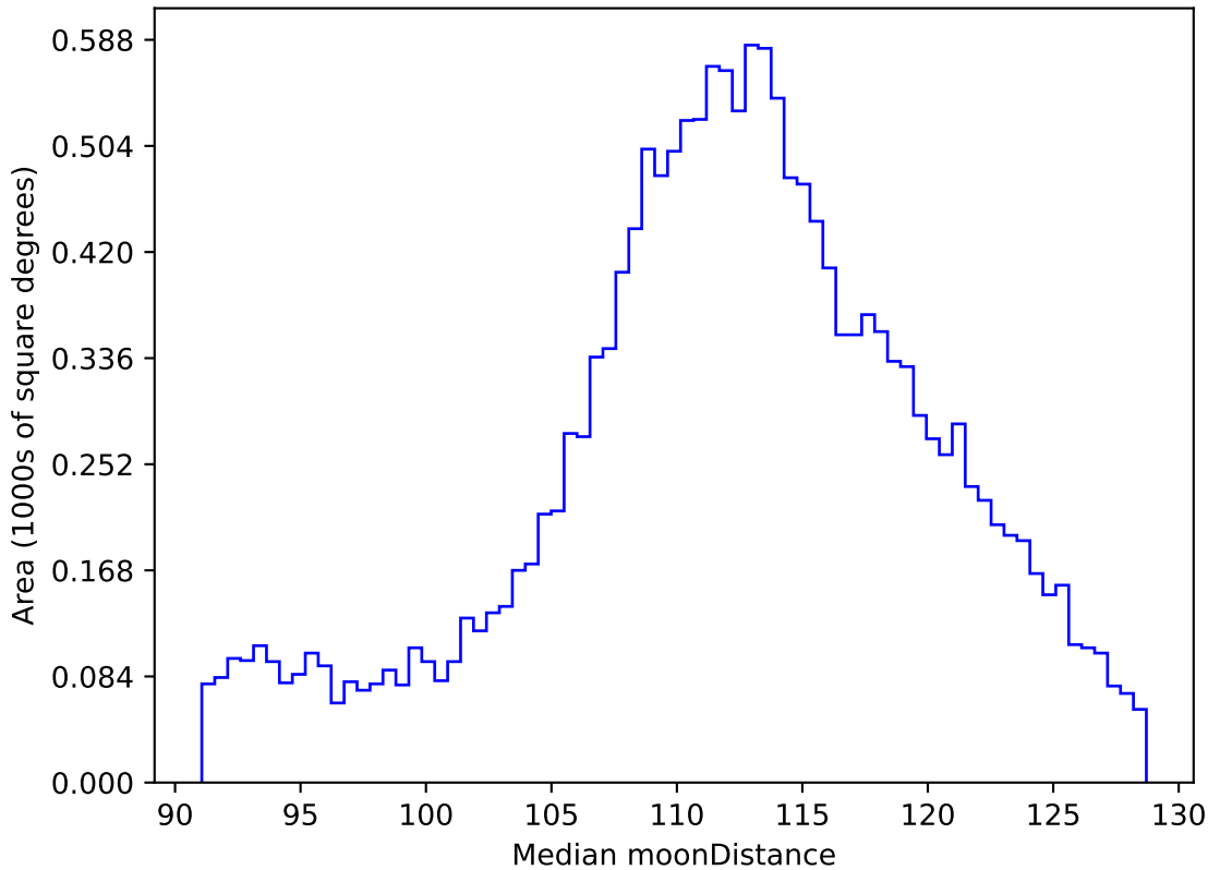
too_elab_r128_d3_ugrizy_v3.4_10yrs WFD r band: Median moonDistance
