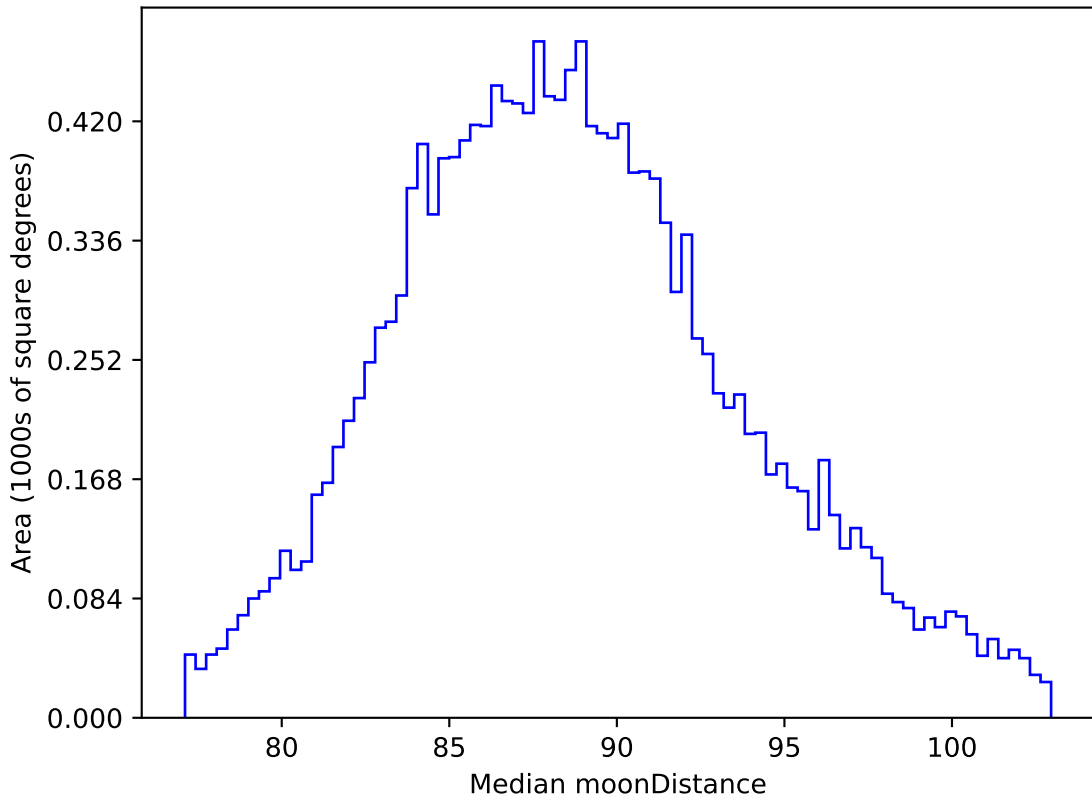
too_elab_r128_d3_ugrizy_v3.4_10yrs WFD all bands: Median moonDistance
