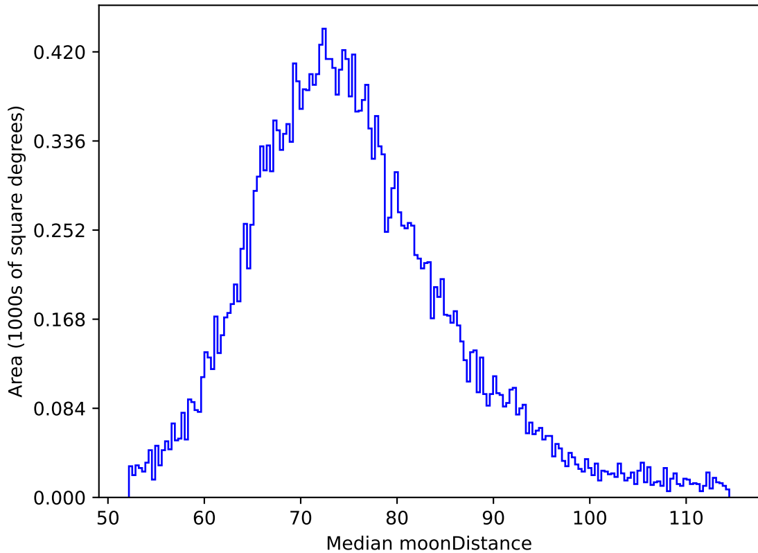
too_elab_r128_d3_ugrizy_v3.4_10yrs All sky z band: Median moonDistance
