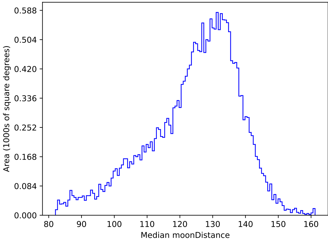
too_elab_r128_d3_ugrizy_v3.4_10yrs All sky u band: Median moonDistance
