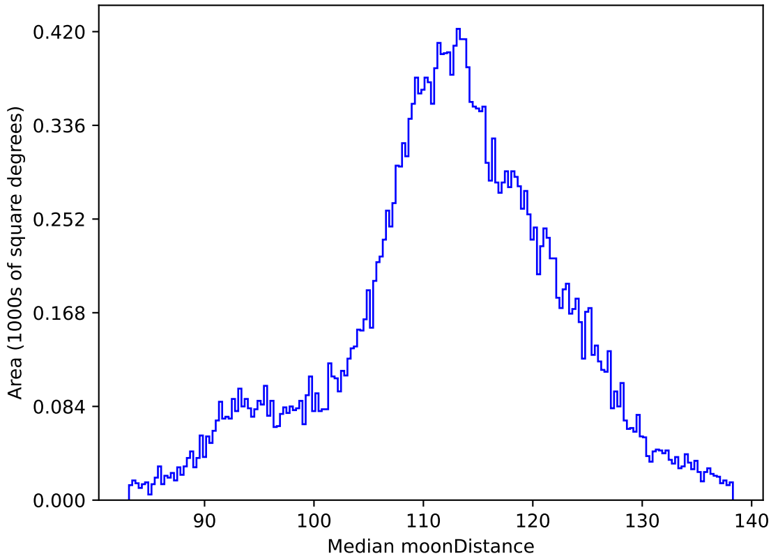
too_elab_r128_d3_ugrizy_v3.4_10yrs All sky r band: Median moonDistance
