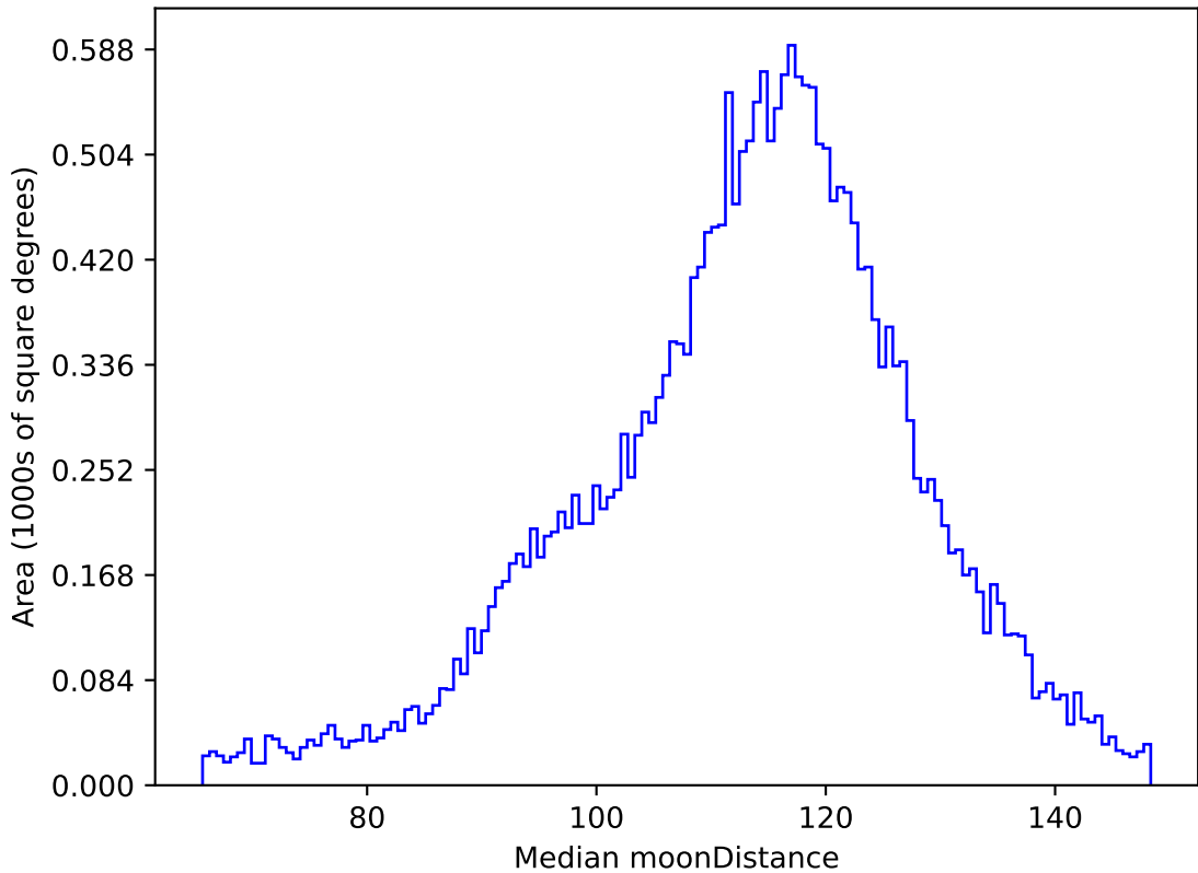
too_elab_r128_d3_ugrizy_v3.4_10yrs All sky g band: Median moonDistance
