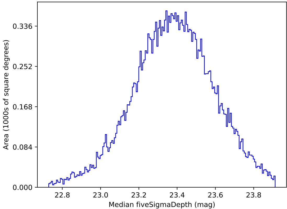
too_elab_r128_d3_ugrizy_v3.4_10yrs Yr 1 all bands: Median fiveSigmaDepth
