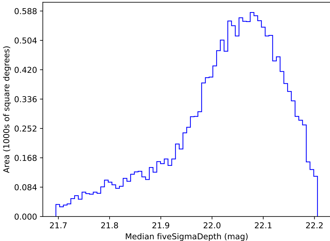
too_elab_r128_d3_ugrizy_v3.4_10yrs WFD y band: Median fiveSigmaDepth
