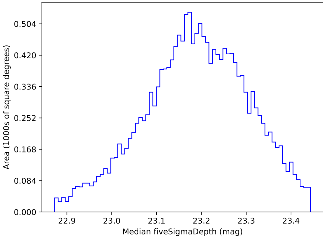
too_elab_r128_d3_ugrizy_v3.4_10yrs WFD u band: Median fiveSigmaDepth
