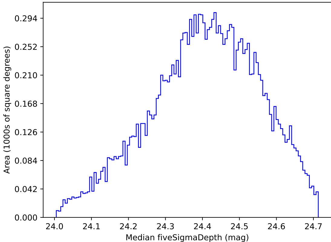
too_elab_r128_d3_ugrizy_v3.4_10yrs WFD g band: Median fiveSigmaDepth
