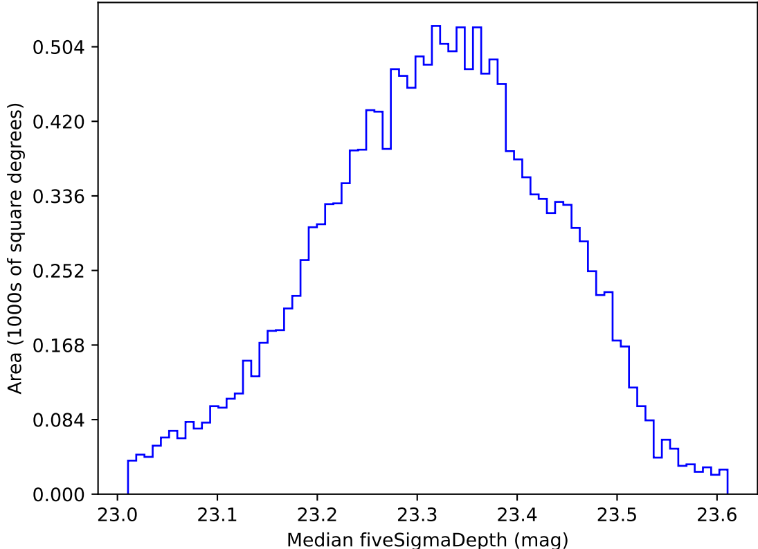
too_elab_r128_d3_ugrizy_v3.4_10yrs WFD all bands: Median fiveSigmaDepth
