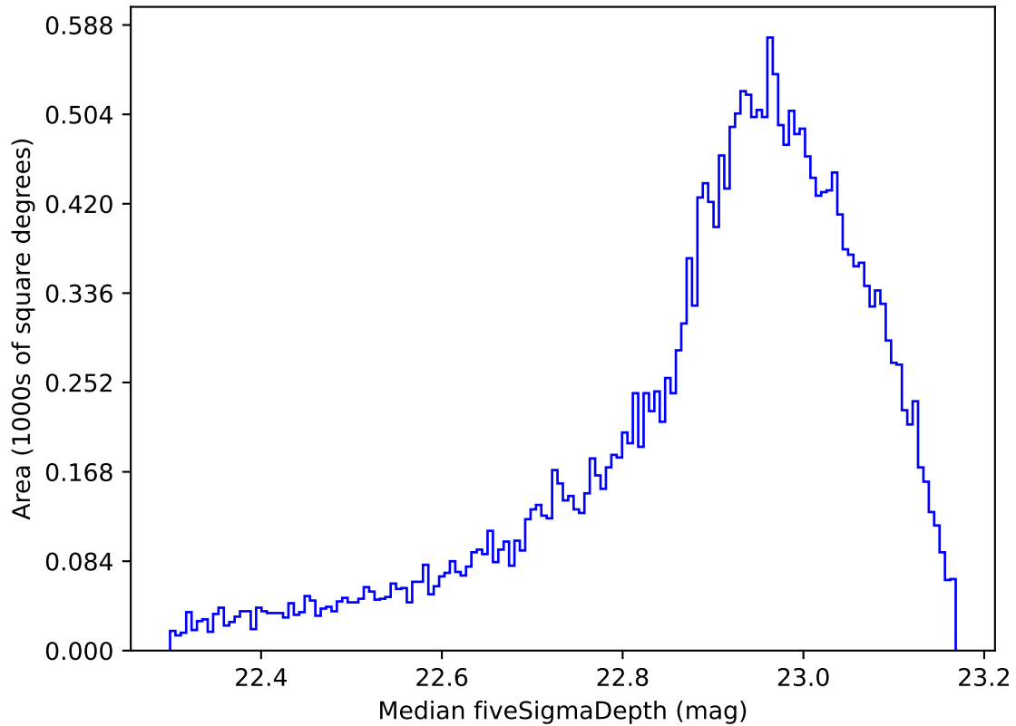
too_elab_r128_d3_ugrizy_v3.4_10yrs All sky z band: Median fiveSigmaDepth
