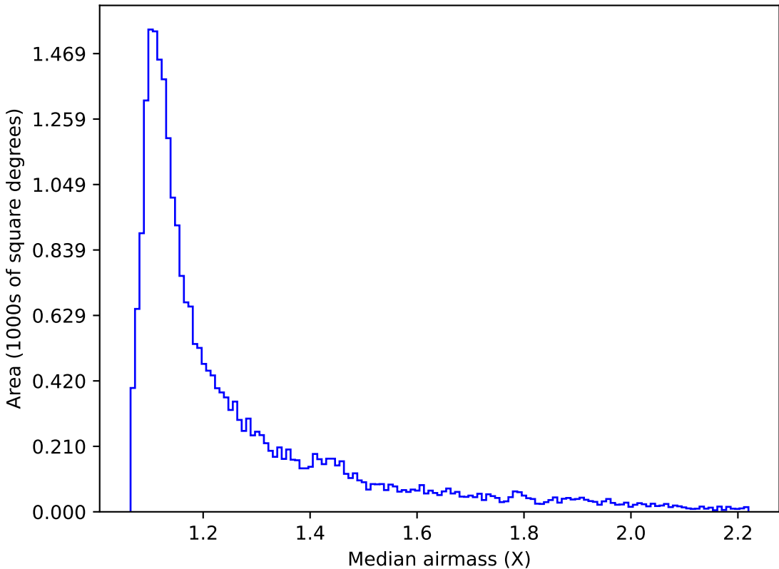
too_elab_r128_d3_ugrizy_v3.4_10yrs Yr 1 z band: Median airmass
