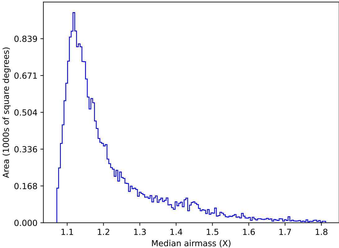
too_elab_r128_d3_ugrizy_v3.4_10yrs Yr 1 y band: Median airmass
