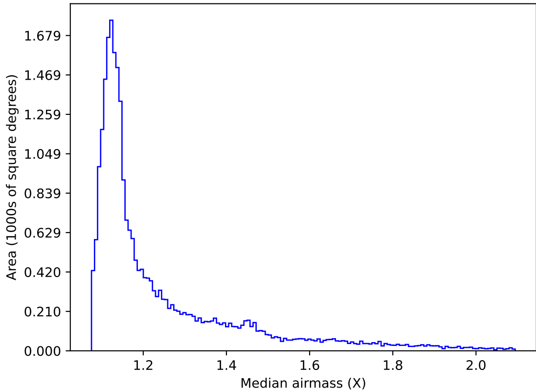
too_elab_r128_d3_ugrizy_v3.4_10yrs Yr 1 all bands: Median airmass
