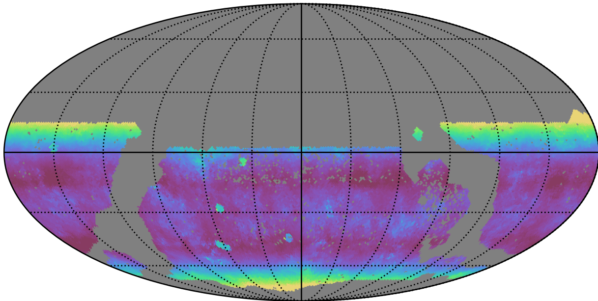
too_elab_r128_d3_ugrizy_v3.4_10yrs WFD z band: Median airmass
