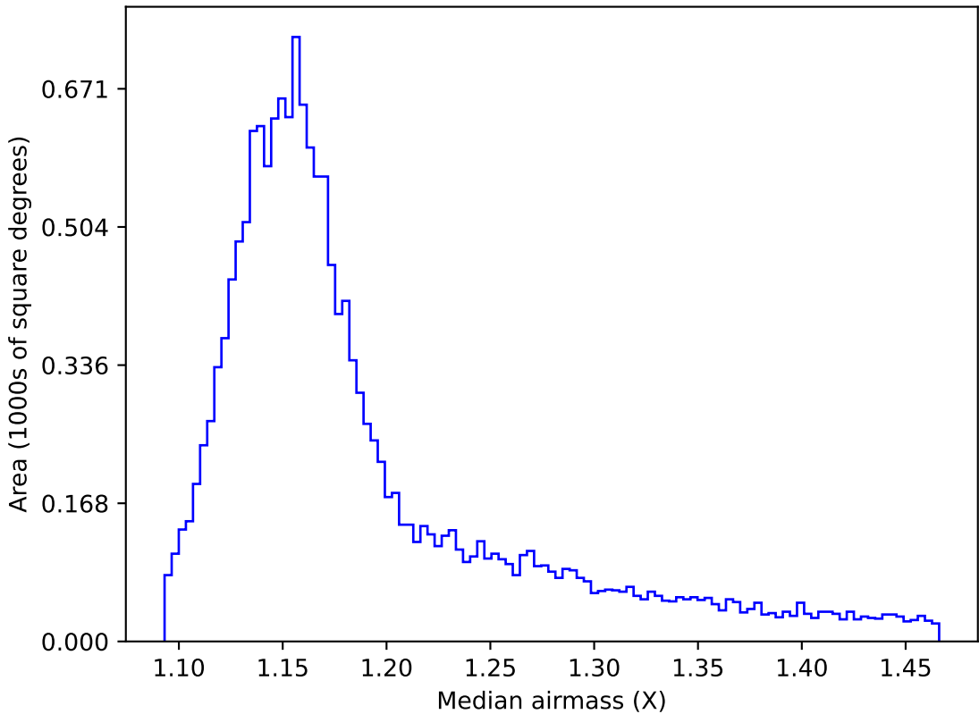
too_elab_r128_d3_ugrizy_v3.4_10yrs WFD z band: Median airmass
