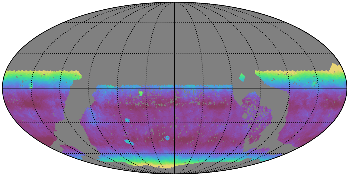
too_elab_r128_d3_ugrizy_v3.4_10yrs WFD y band: Median airmass
