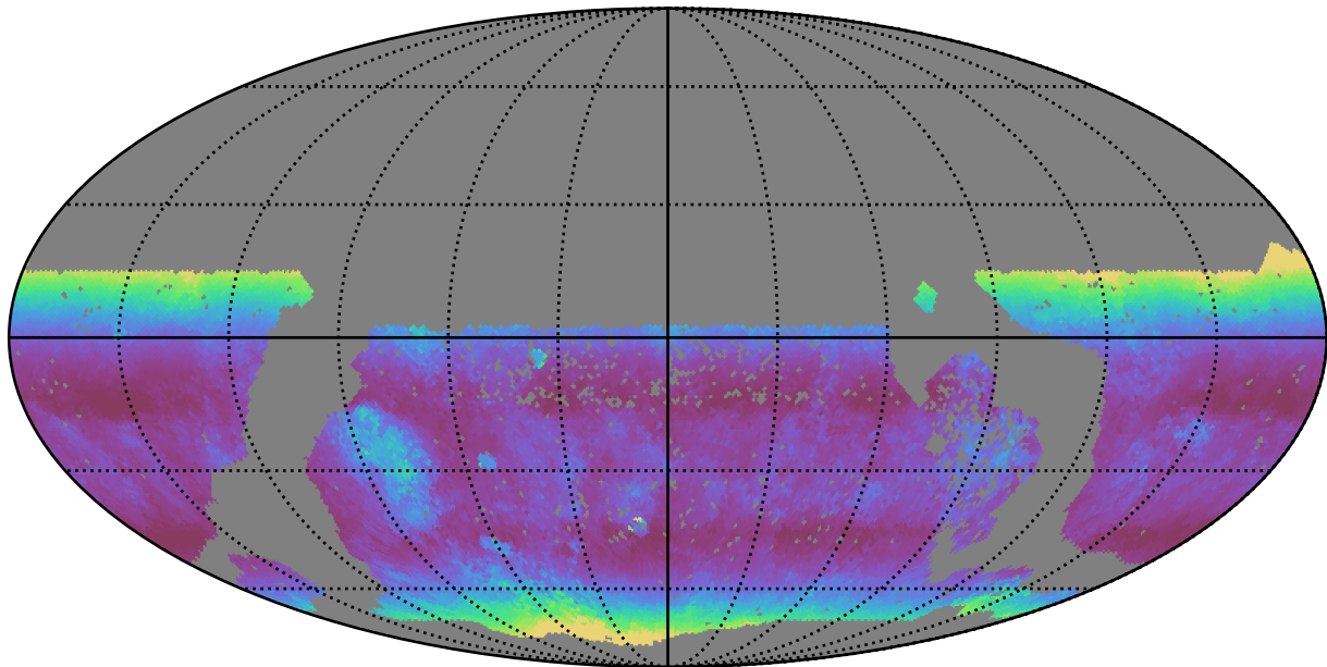
too_elab_r128_d3_ugrizy_v3.4_10yrs WFD u band: Median airmass
