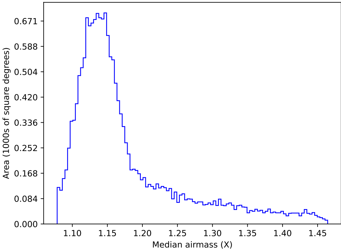
too_elab_r128_d3_ugrizy_v3.4_10yrs WFD r band: Median airmass
