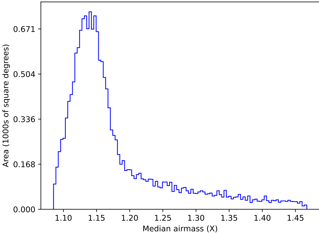
too_elab_r128_d3_ugrizy_v3.4_10yrs WFD i band: Median airmass
