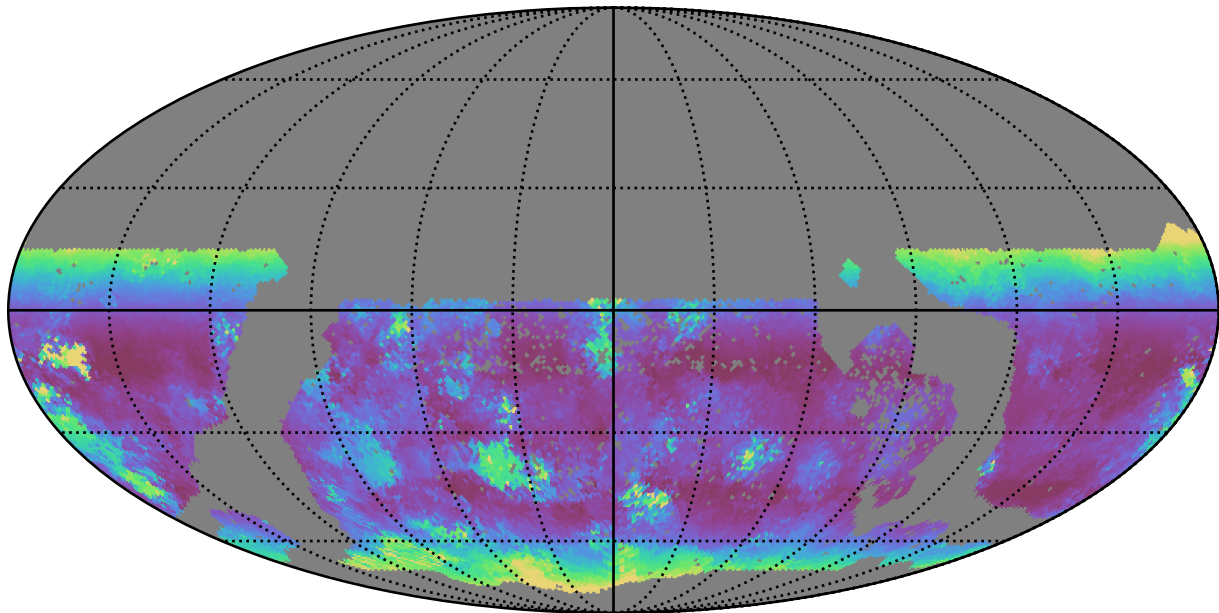
too_elab_r128_d3_ugrizy_v3.4_10yrs WFD g band: Median airmass
