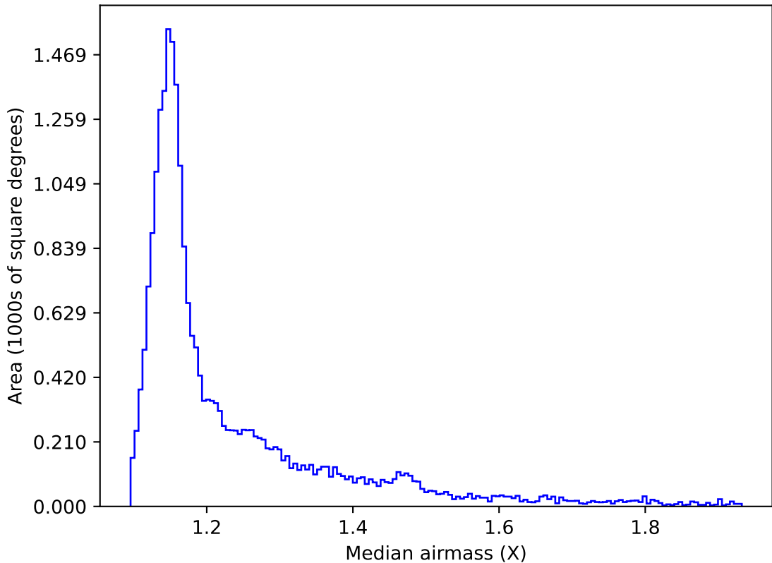
too_elab_r128_d3_ugrizy_v3.4_10yrs All sky y band: Median airmass
