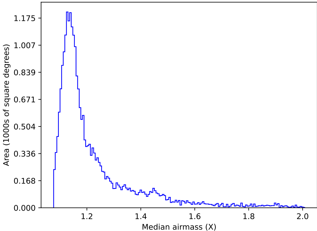
too_elab_r128_d3_ugrizy_v3.4_10yrs All sky u band: Median airmass
