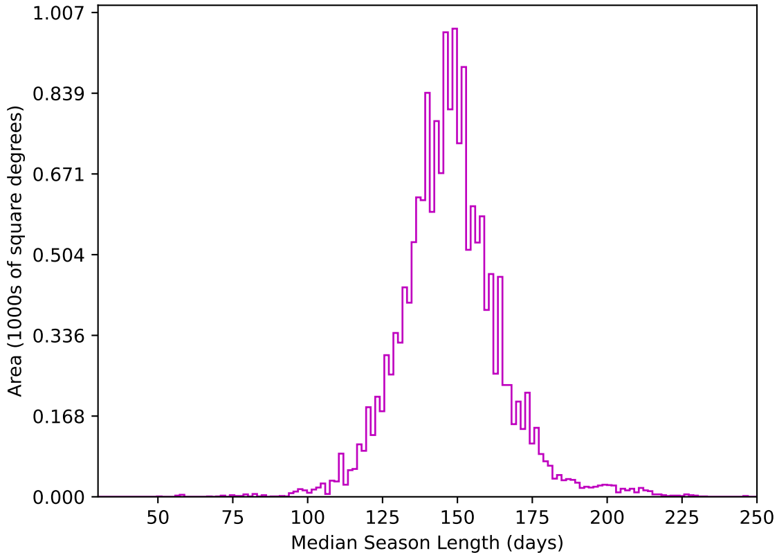
too_elab_r128_d3_ugrizy_v3.4_10yrs WFD z band: Median Season Length
