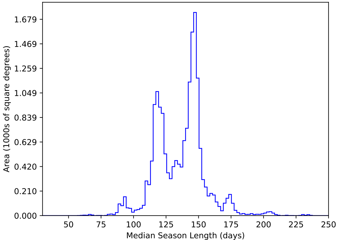
too_elab_r128_d3_ugrizy_v3.4_10yrs WFD y band: Median Season Length
