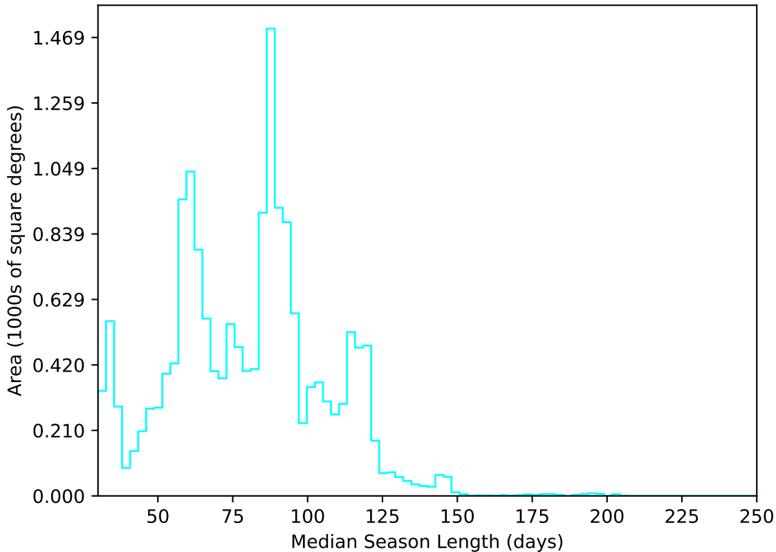
too_elab_r128_d3_ugrizy_v3.4_10yrs WFD u band: Median Season Length
