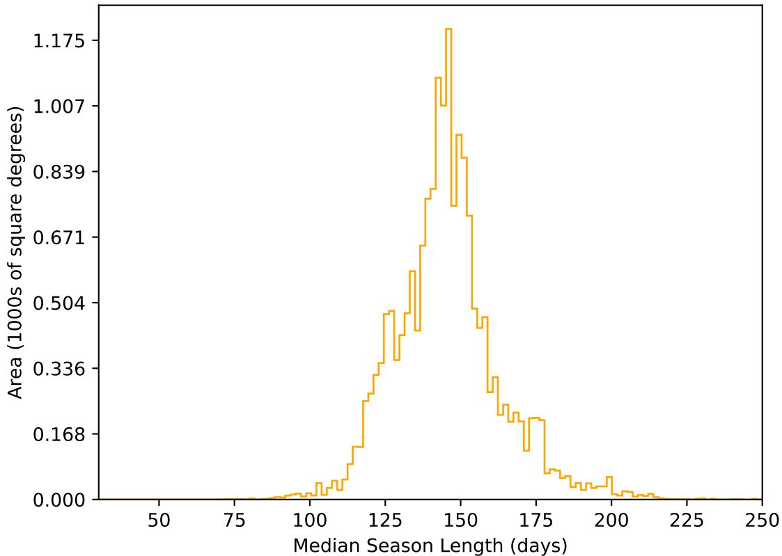
too_elab_r128_d3_ugrizy_v3.4_10yrs WFD r band: Median Season Length
