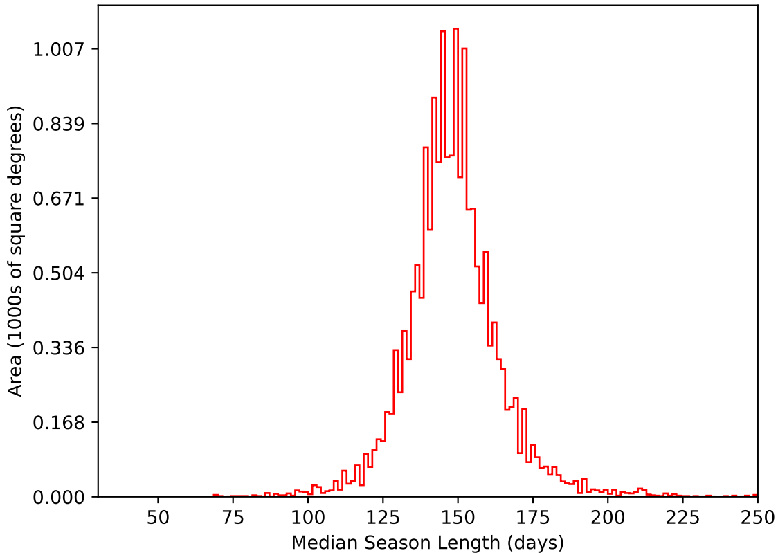
too_elab_r128_d3_ugrizy_v3.4_10yrs WFD i band: Median Season Length
