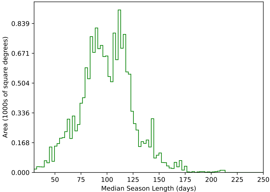
too_elab_r128_d3_ugrizy_v3.4_10yrs WFD g band: Median Season Length
