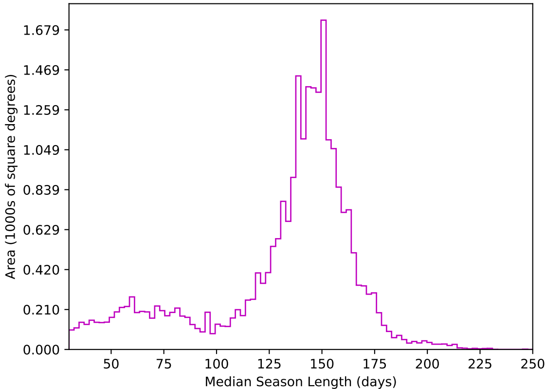
too_elab_r128_d3_ugrizy_v3.4_10yrs All sky z band: Median Season Length
